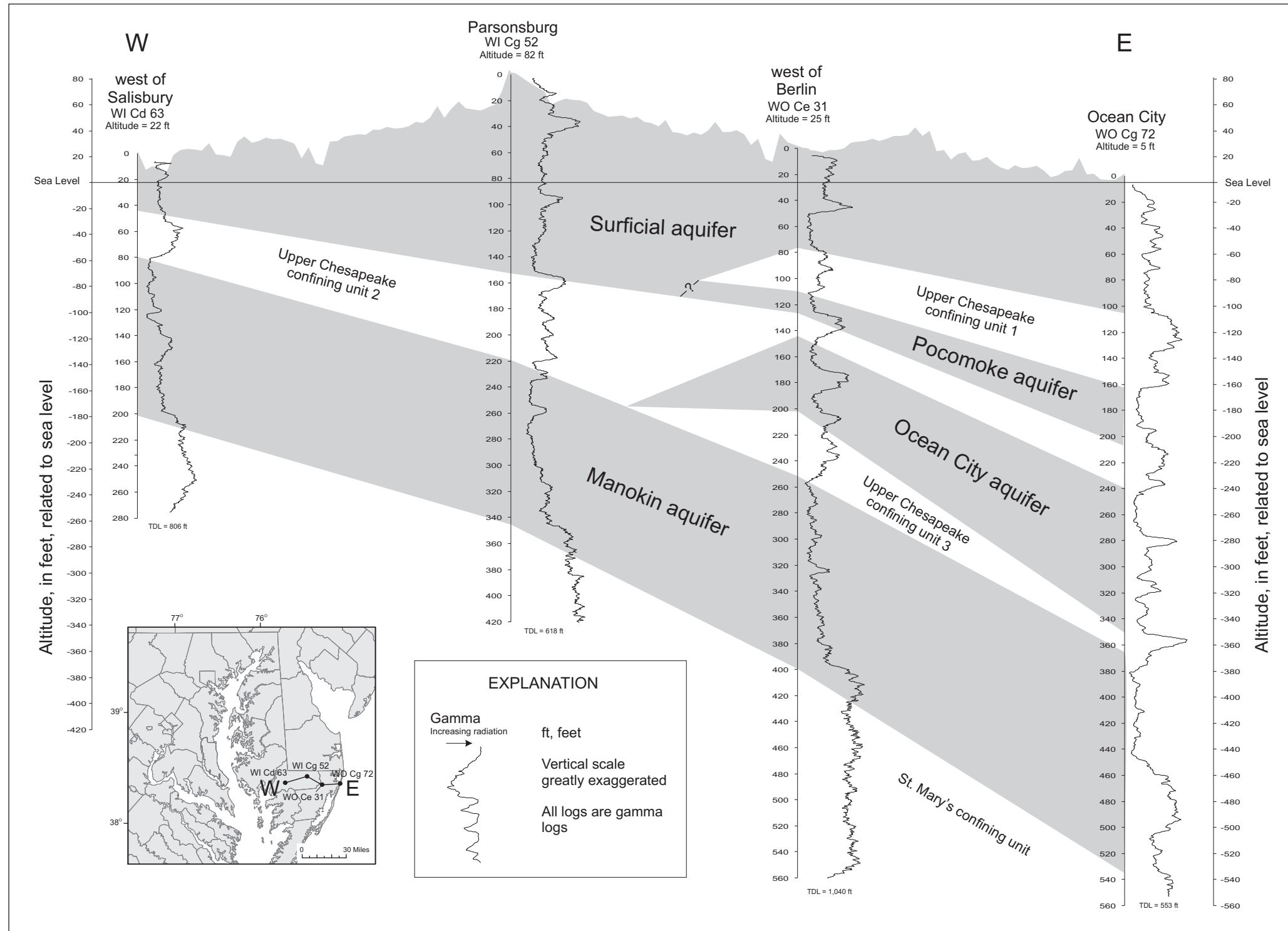
Hydrogeologic cross section showing the Pocomoke, Ocean City, Manokin and Surficial aquifers on the Eastern Shore of Maryland.
